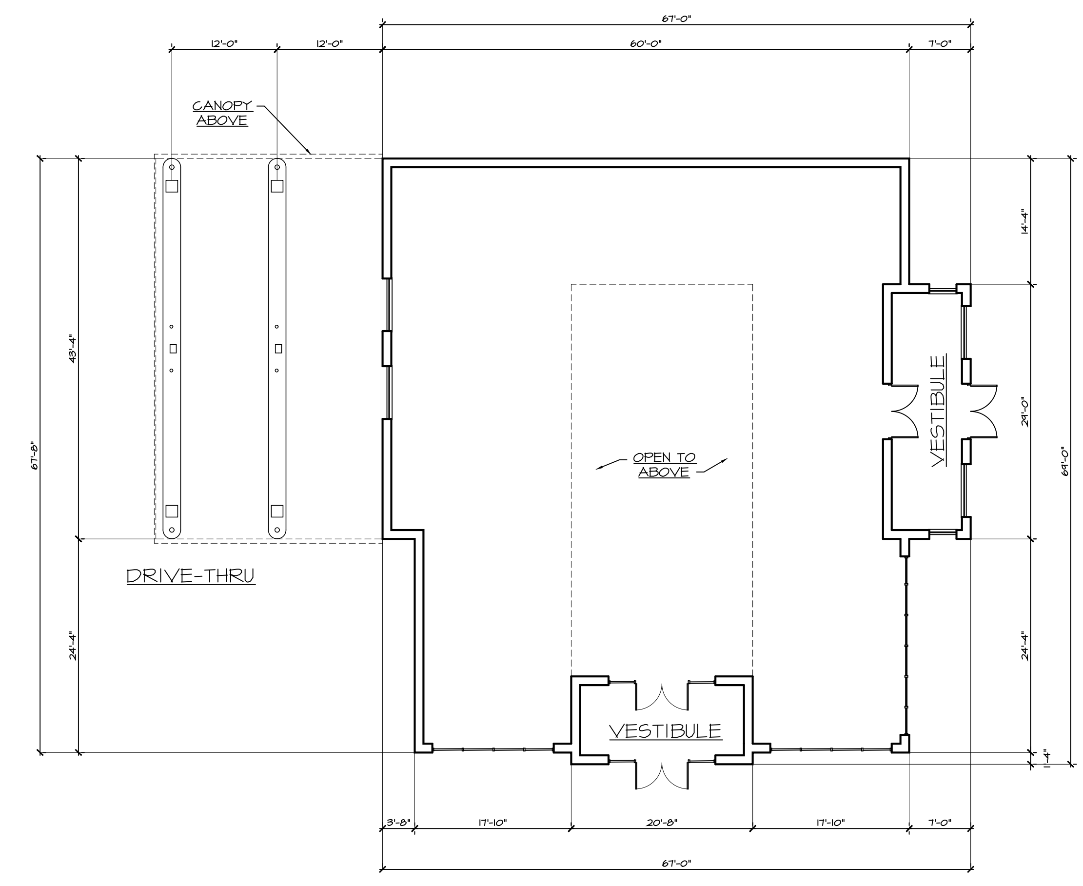
1 FIRST FLOOR PLAN AS.0E SCALE: 3/32" = 1'-0" 4,201 GSF
